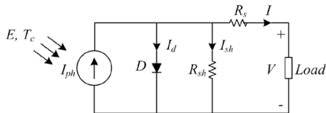
2 FIGURE 2. Electric circuit of modeling of solar cell
