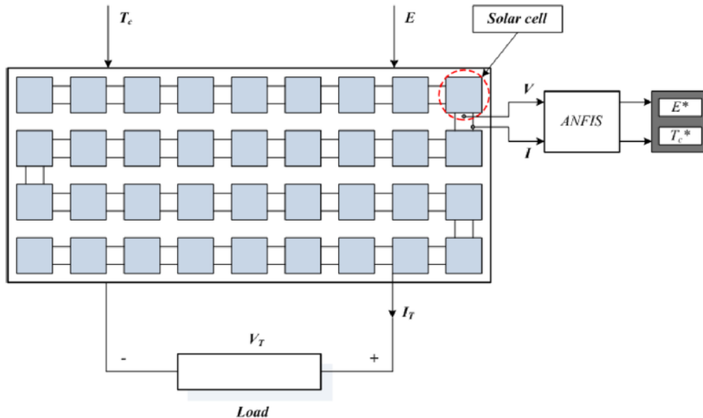
19 FIGURE 1. Configuration of the proposed system
